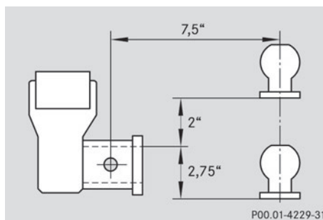
Ball position of the ball coupling
